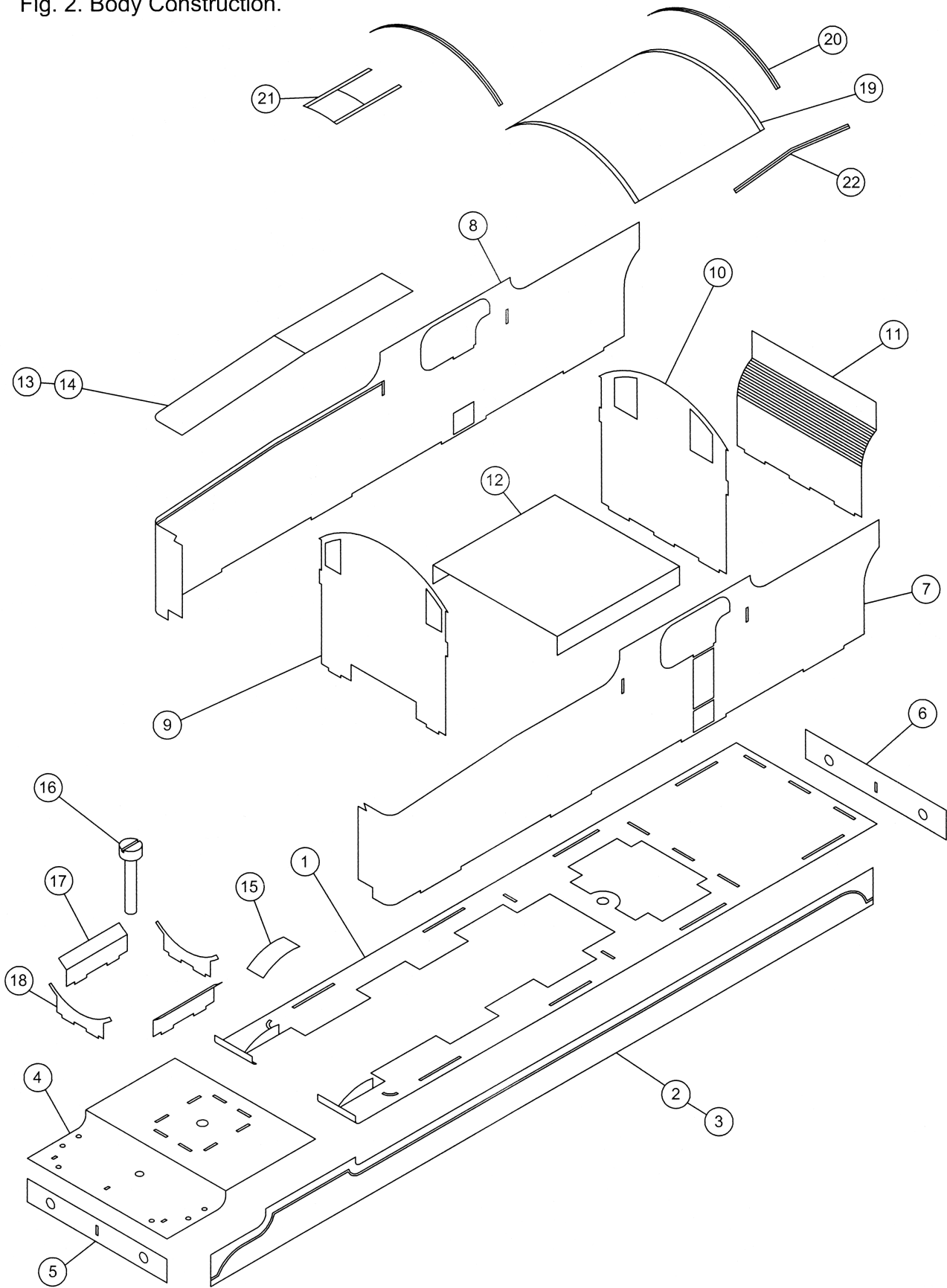
Fig. 2. Body Construction.
